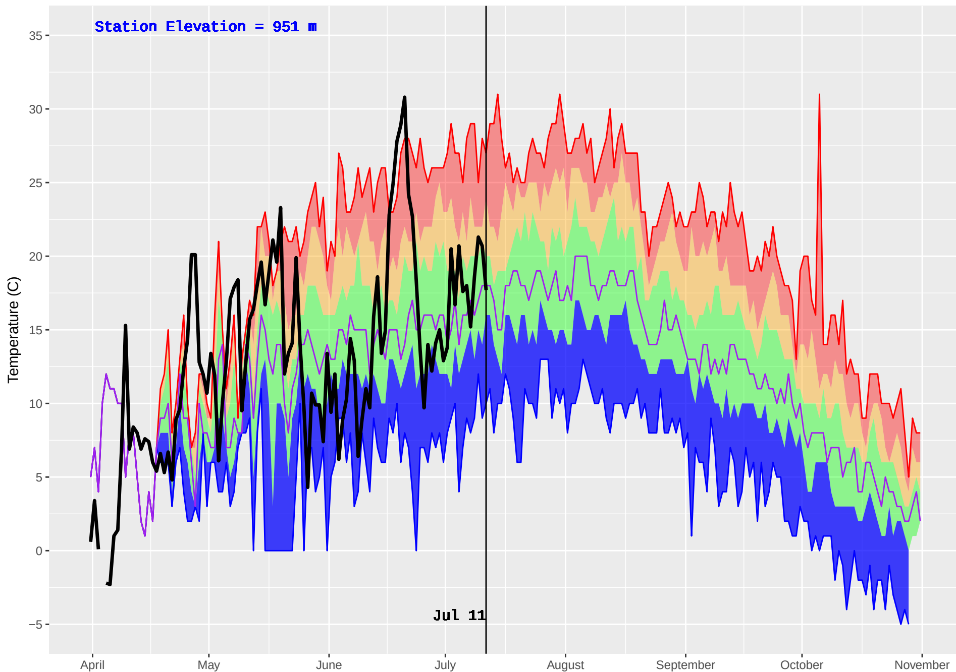
NORTH BABINE (173) : Historical (1986–2016) and Current (2018) Noon Temperature
