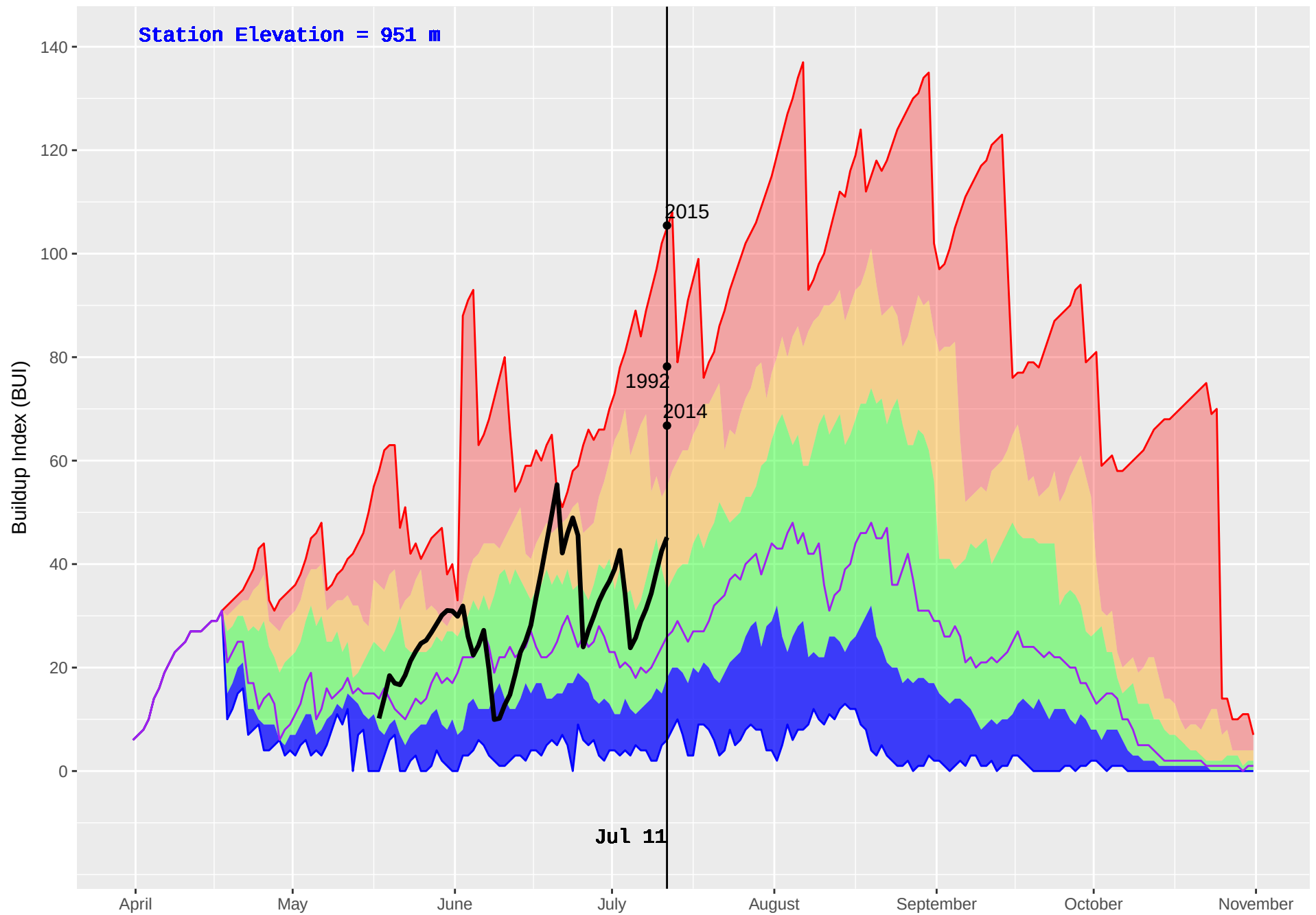
NORTH BABINE (173) : Historical (1986–2016) and Current (2018) Noon Buildup Index (BUI)
