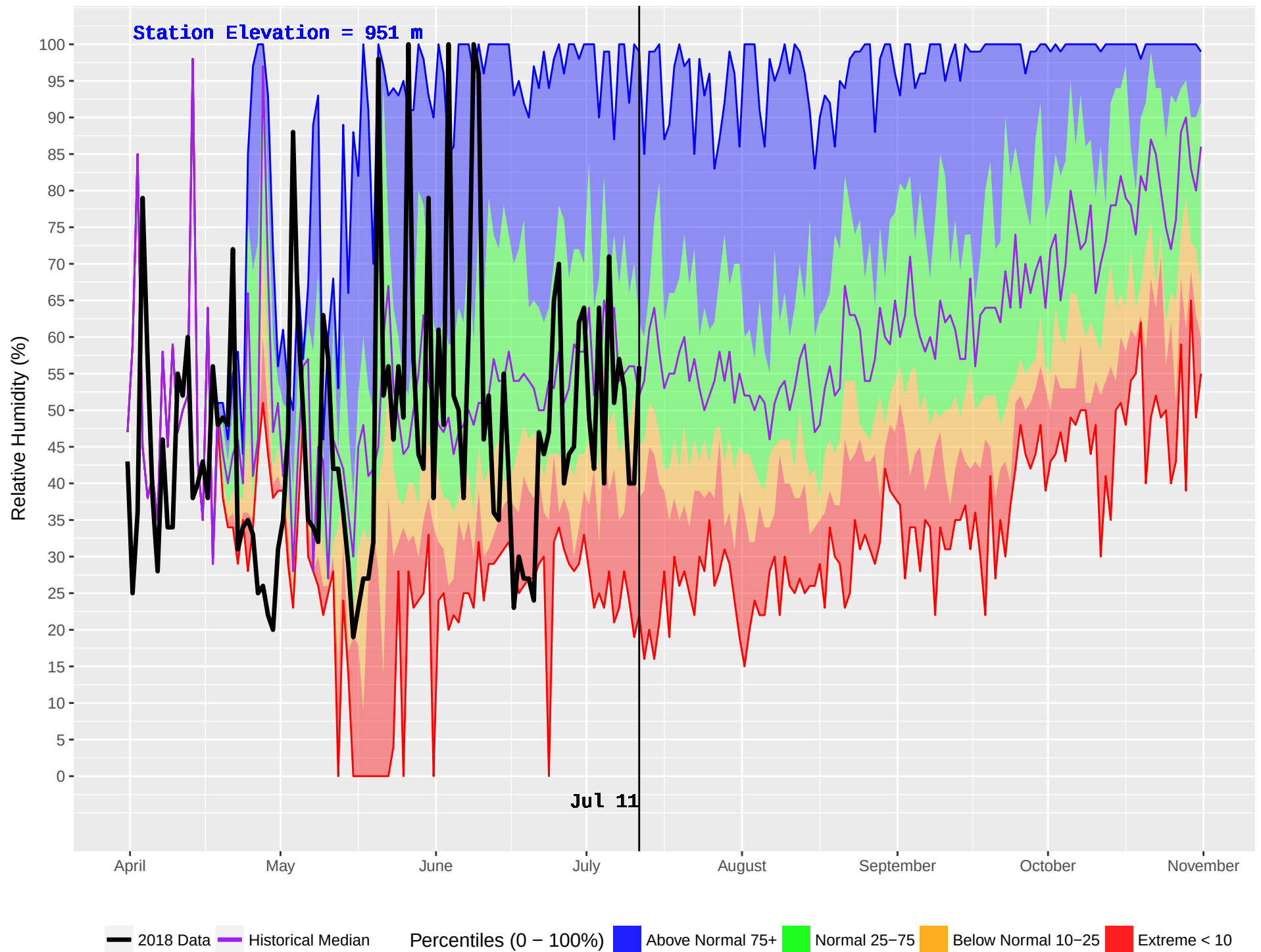
NORTH BABINE (173) : Historical (1986–2016) and Current (2018) Noon Relative Humidity
